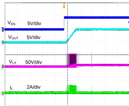
Startup from EN ( V_{IN}=48V , V_{OUT}=5V , I_{OUT}=0A )
