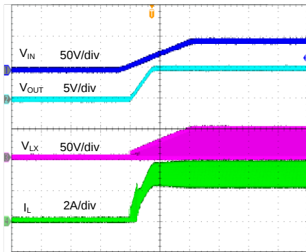
Startup from V_{IN} ( V_{IN}=48V , V_{OUT}=5V , I_{OUT}=3A )
