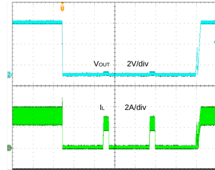
Short Circuit Protection ( V_{IN}=48V , V_{OUT}=5V , I_{OUT}=3A -short)
