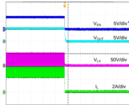
Shutdown from EN ( V_{IN}=48V , V_{OUT}=5V , I_{OUT}=3A )
