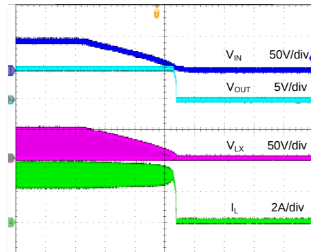
Shutdown from V_{IN} ( V_{IN}=48V , V_{OUT}=5V , I_{OUT}=3A )
