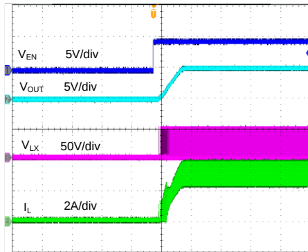
Startup from EN ( V_{IN}=48V , V_{OUT}=5V , I_{OUT}=3A )
