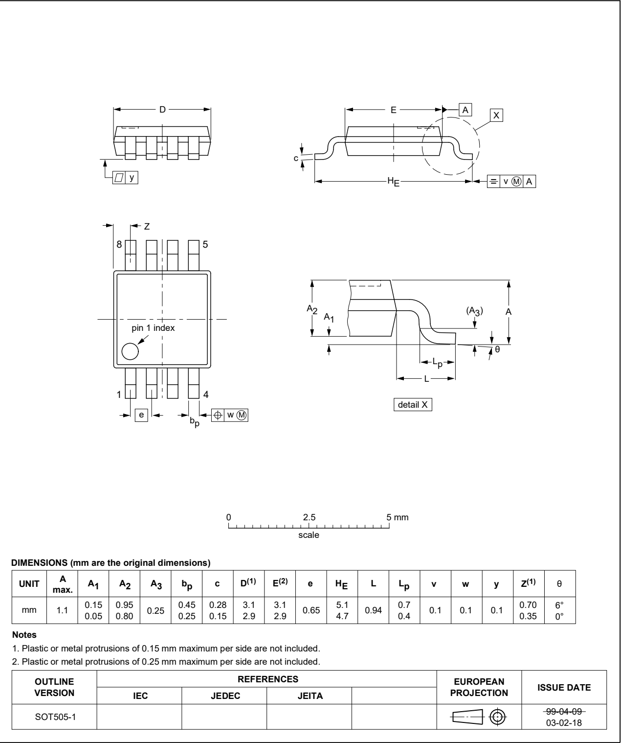
Figure 34. Package outline SOT505-1 (TSSOP8) of PCF85063ATT
